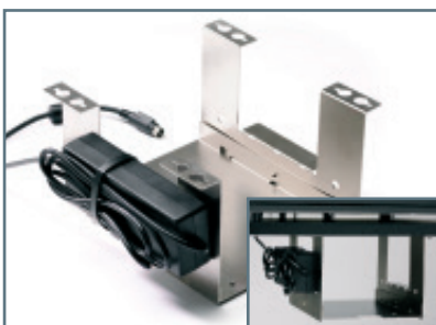
Under Shelf Mount option with power supply holder
